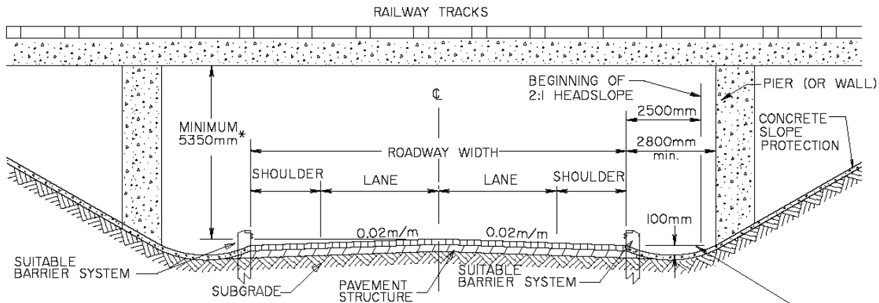
FIGURE H7.3 Minimum Clearance Requirements For Railway Underpass and Grade Separations (See Typical Details on Figure H7.1)
