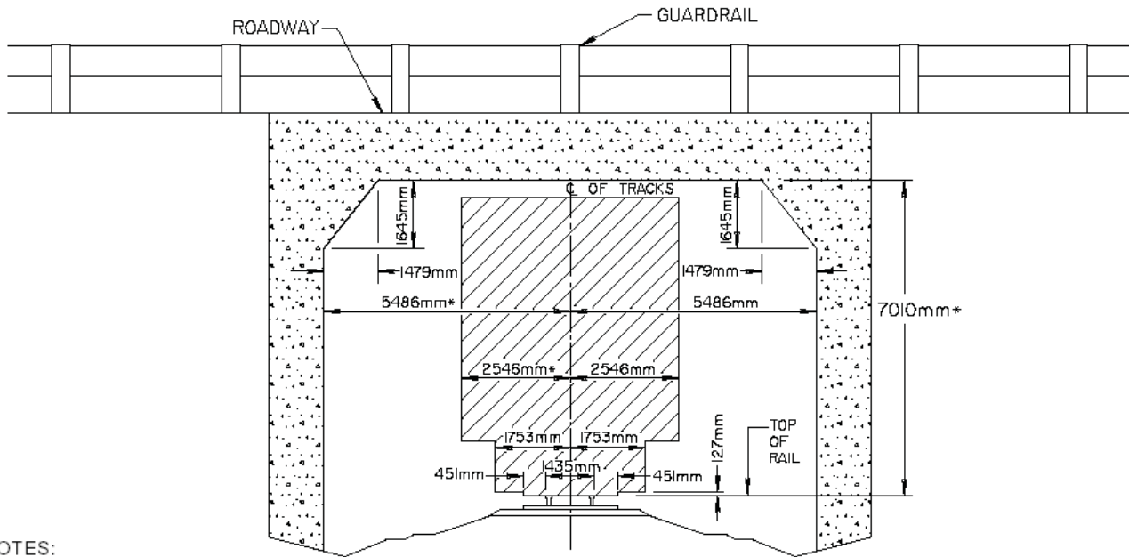
FIGURE H7.2 Minimum Clearance Requirements For Railway Overpass
